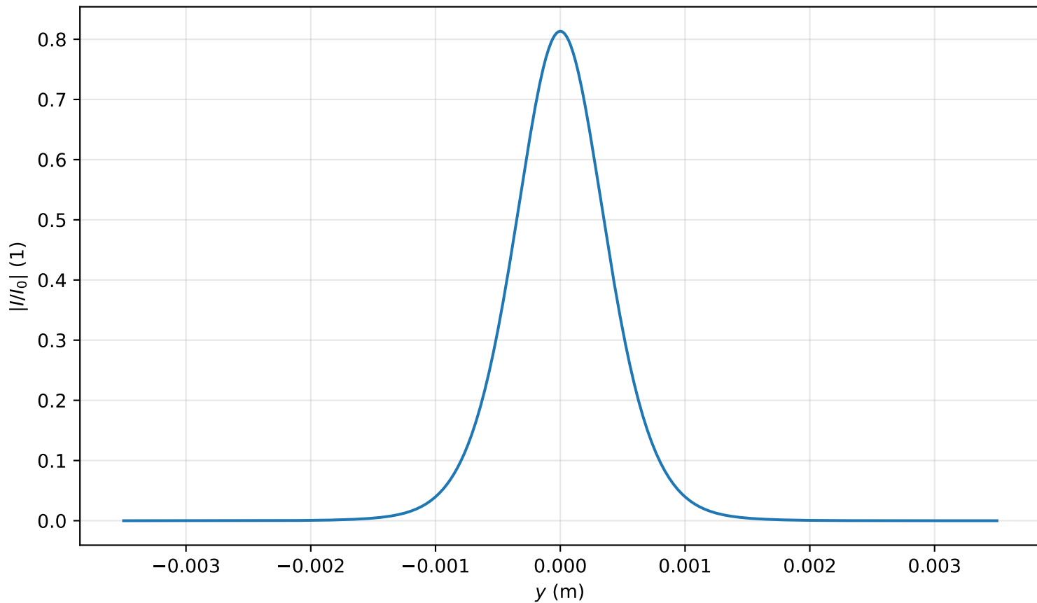
Intensity profile I(x = 0, y, z = 2.468)/I_0 , P_{in}=0.6P_{cr} , artificial time
